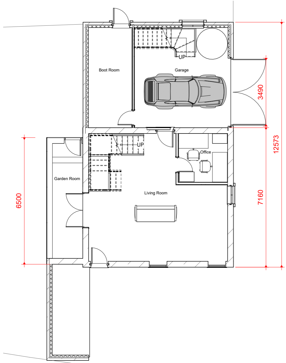
1 0 PROPOSED GROUND FLOOR 1 : 50
