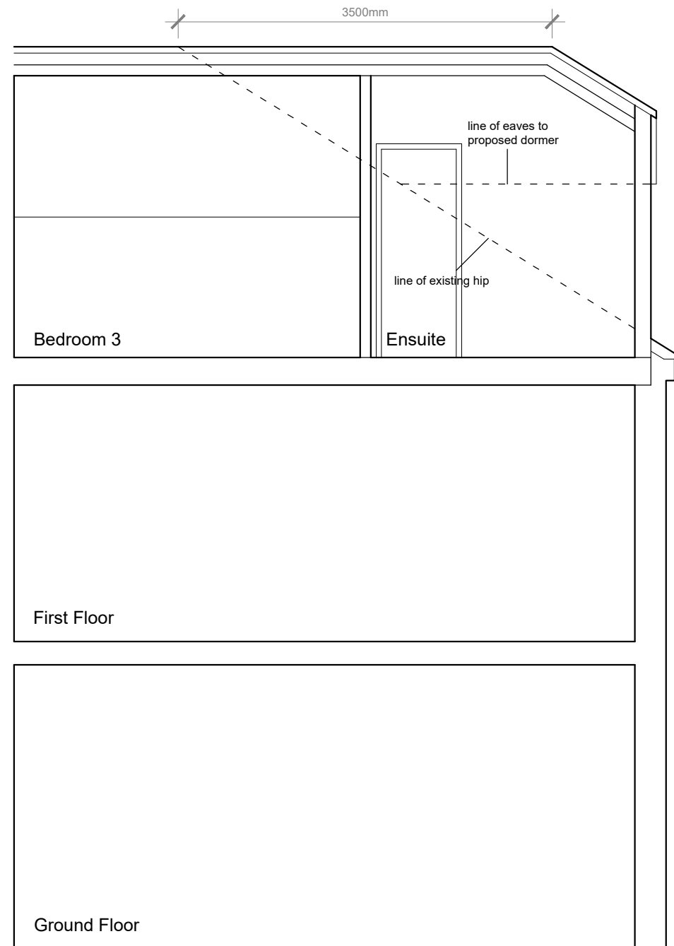
Section BB Thro' Proposed Dormer
