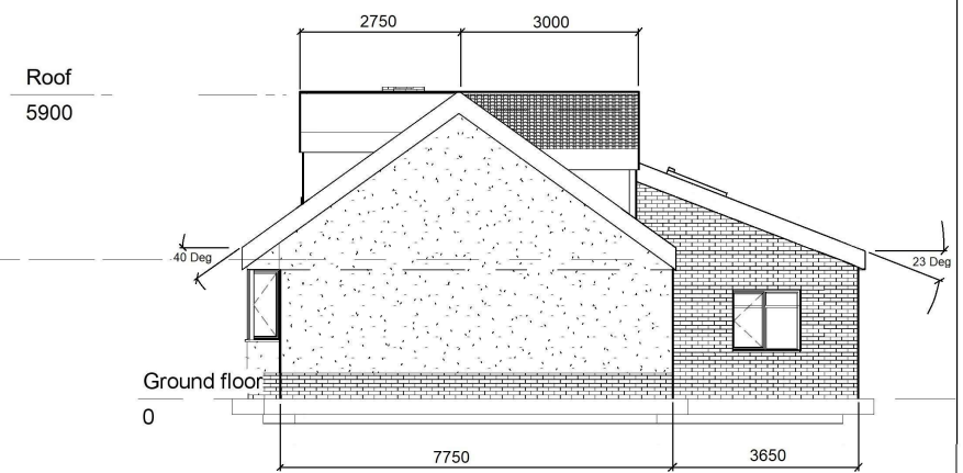
Proposed Side Elevation - RH (3)
