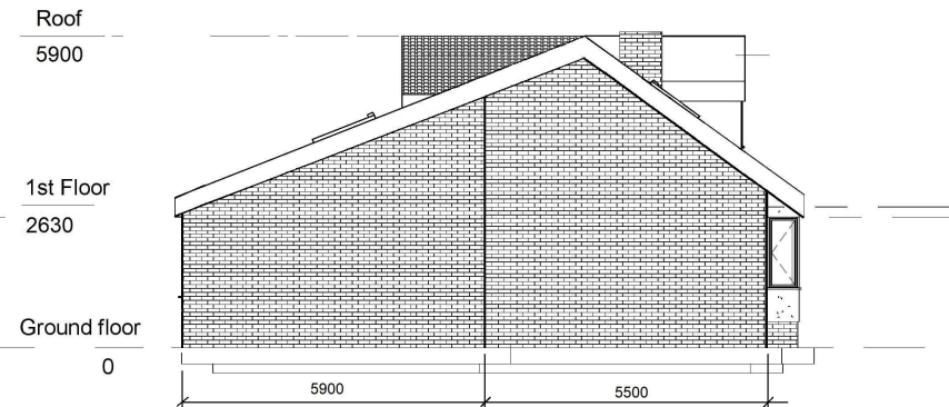
Proposed Side Elevation - LH (4)
