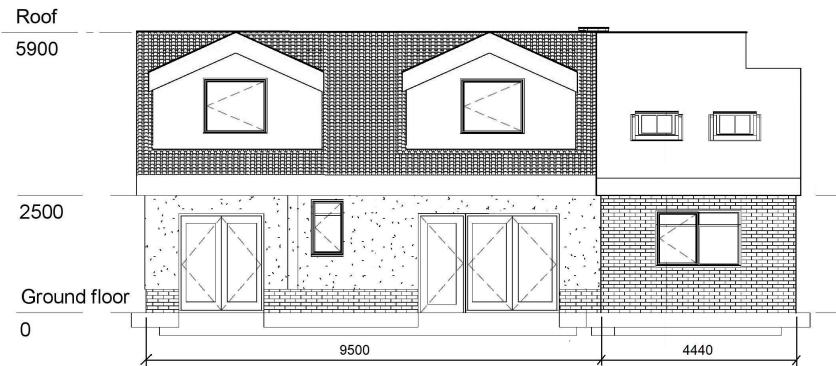
Proposed Rear Elevation (2)
