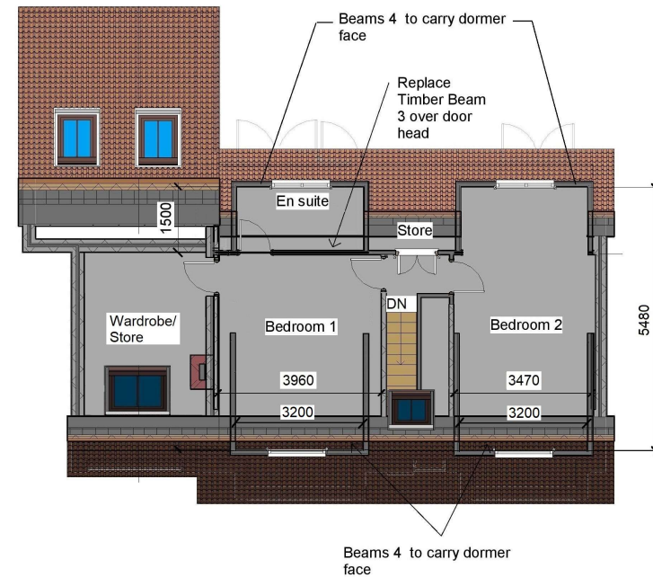
First Floor Section (2)
