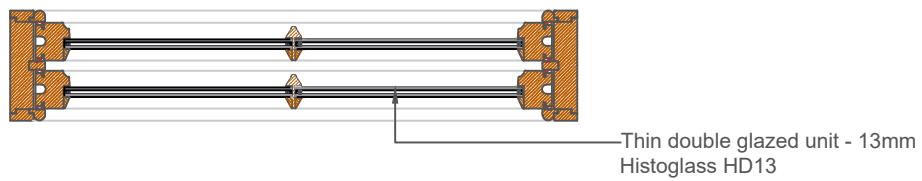
Proposed Sash Window Details 1:10
