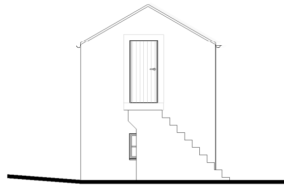
Outbuilding South Elevation 1 : 100
