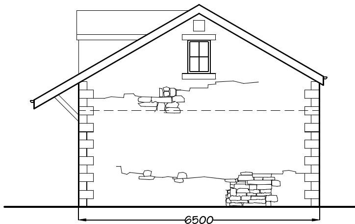
South Elevation
