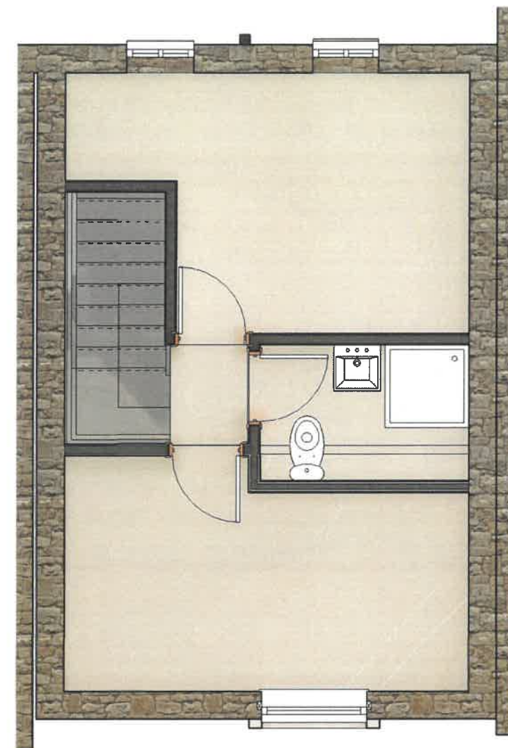
2 SECOND FLOOR 1 : 25
