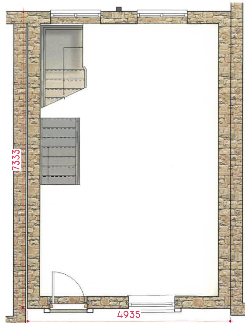
1 FIRST FLOOR 1 : 25
