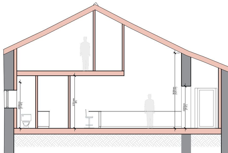
PROPOSED SECTION C-C
