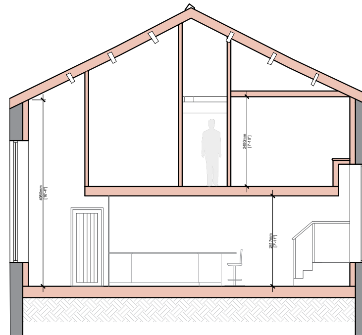
PROPOSED SECTION B-B
