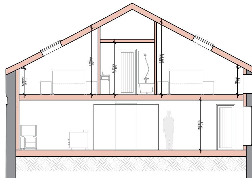
PROPOSED SECTION D-D
