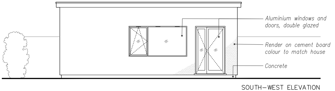
SOUTH-WEST ELEVATION
