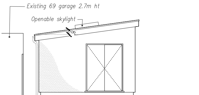
NORTH-WEST ELEVATION
