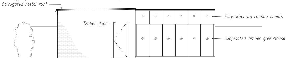
SOUTH-WEST ELEVATION
