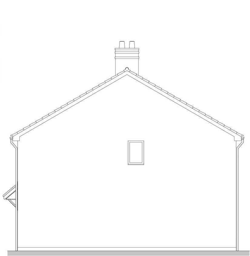
Side Elevation
