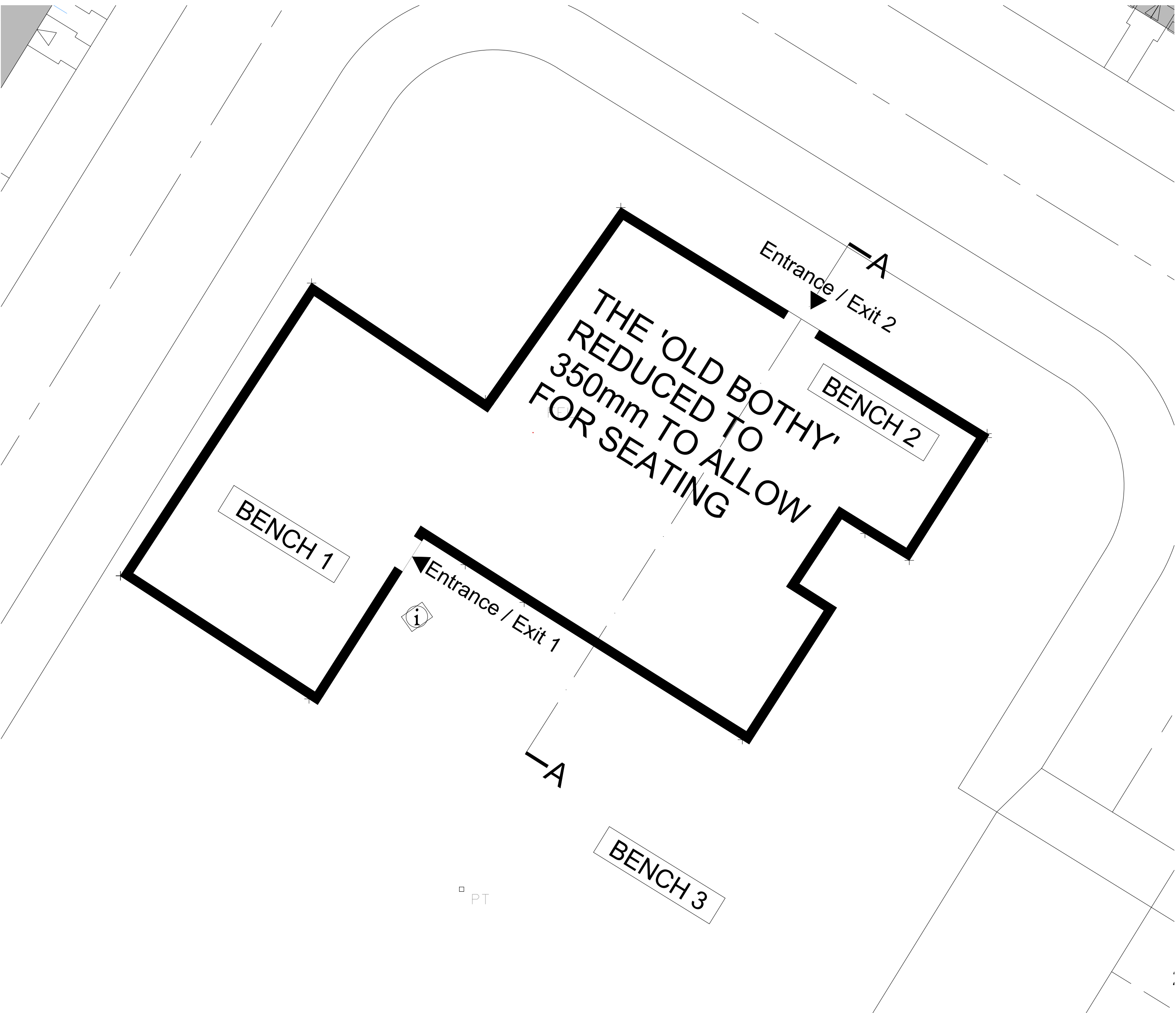
Bothy Plan [1:100]
