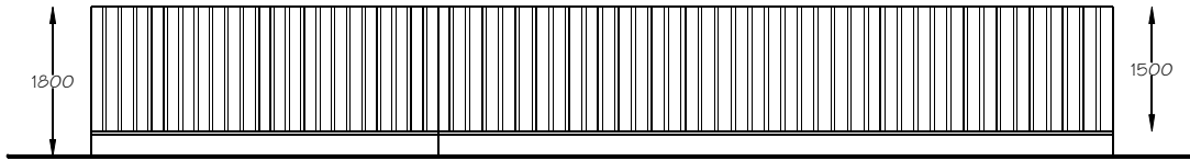
west elevation
