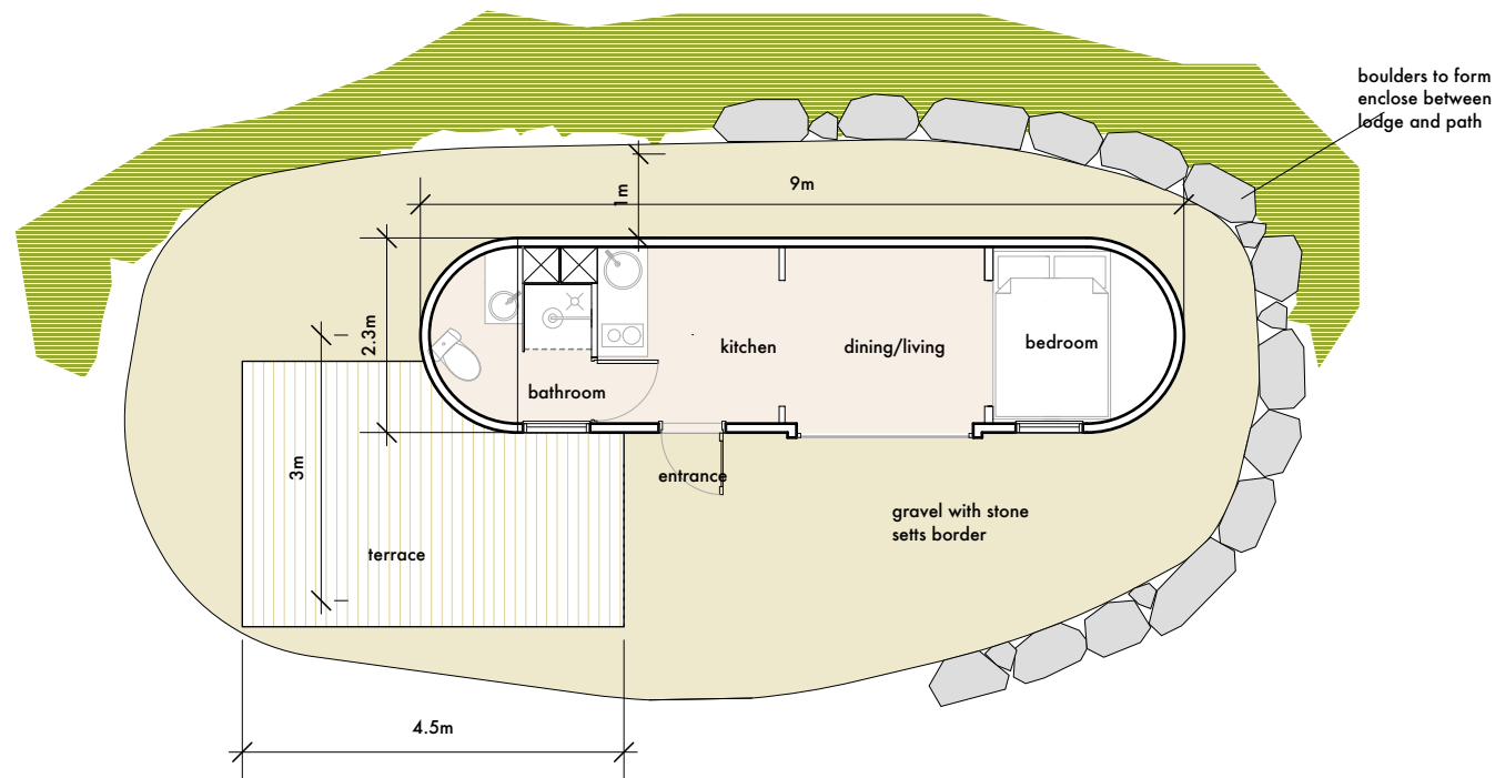
floor plan
