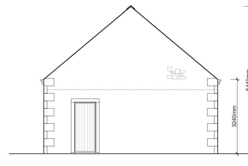
PROPOSED PLOT 2 GARAGE EAST ELEVATION Scale 1:100
