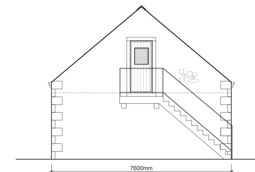
PROPOSED PLOT 2 GARAGE WEST ELEVATION Scale 1:100
