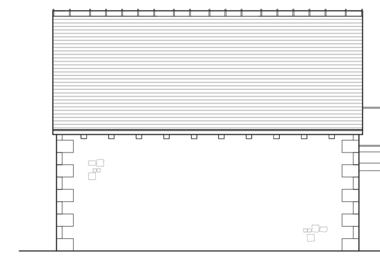
PROPOSED PLOT 2 GARAGE NORTH ELEVATION Scale 1:100
