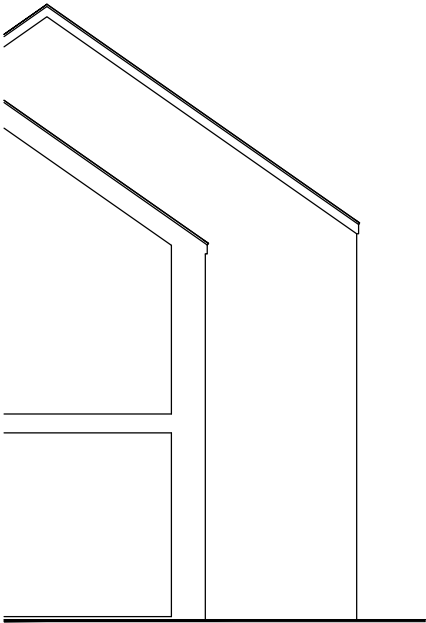
EXSITING SIDE SECTIONAL ELEVATION B 1:100
