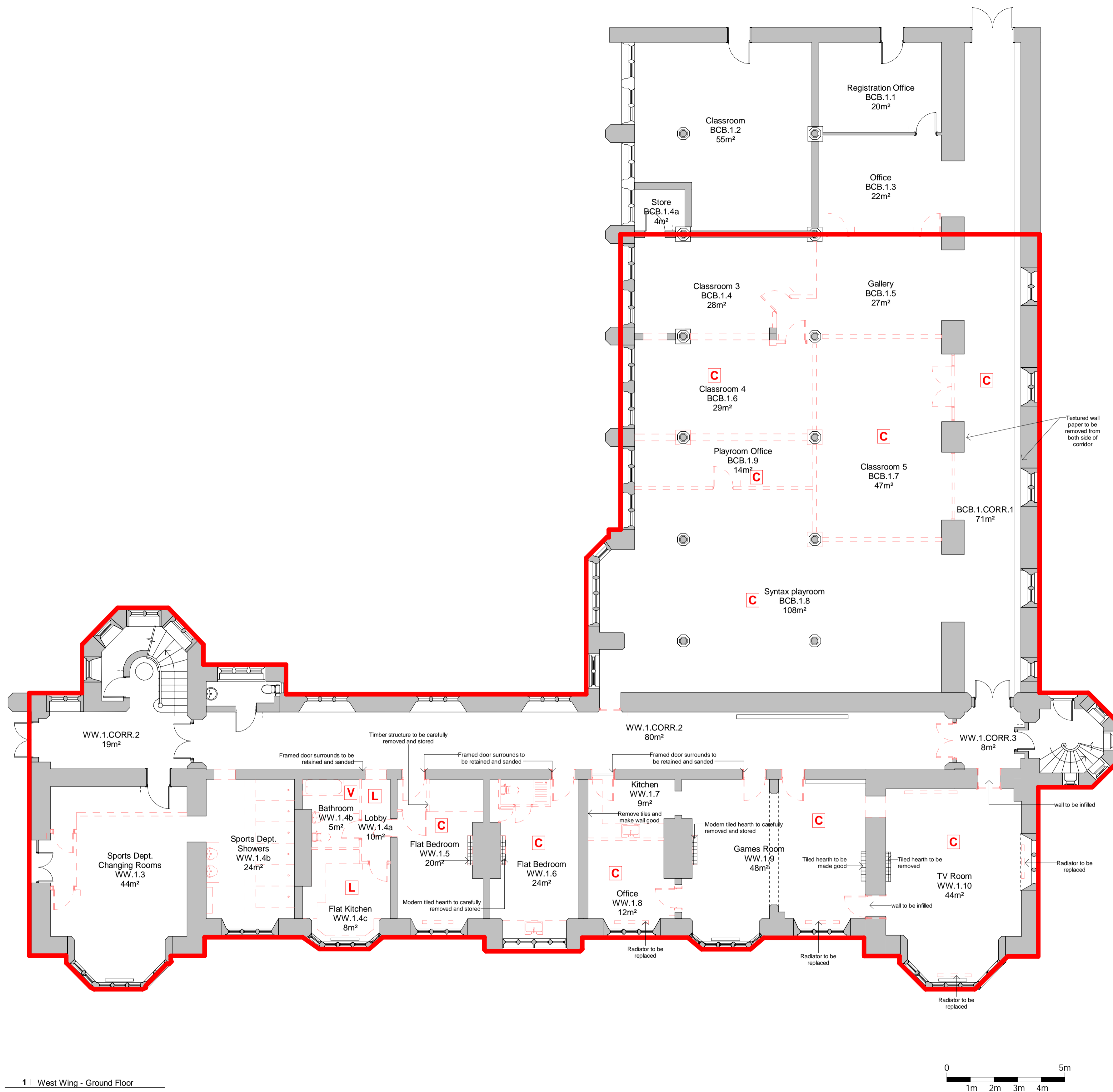
1 | West Wing - Ground Floor 1:100
