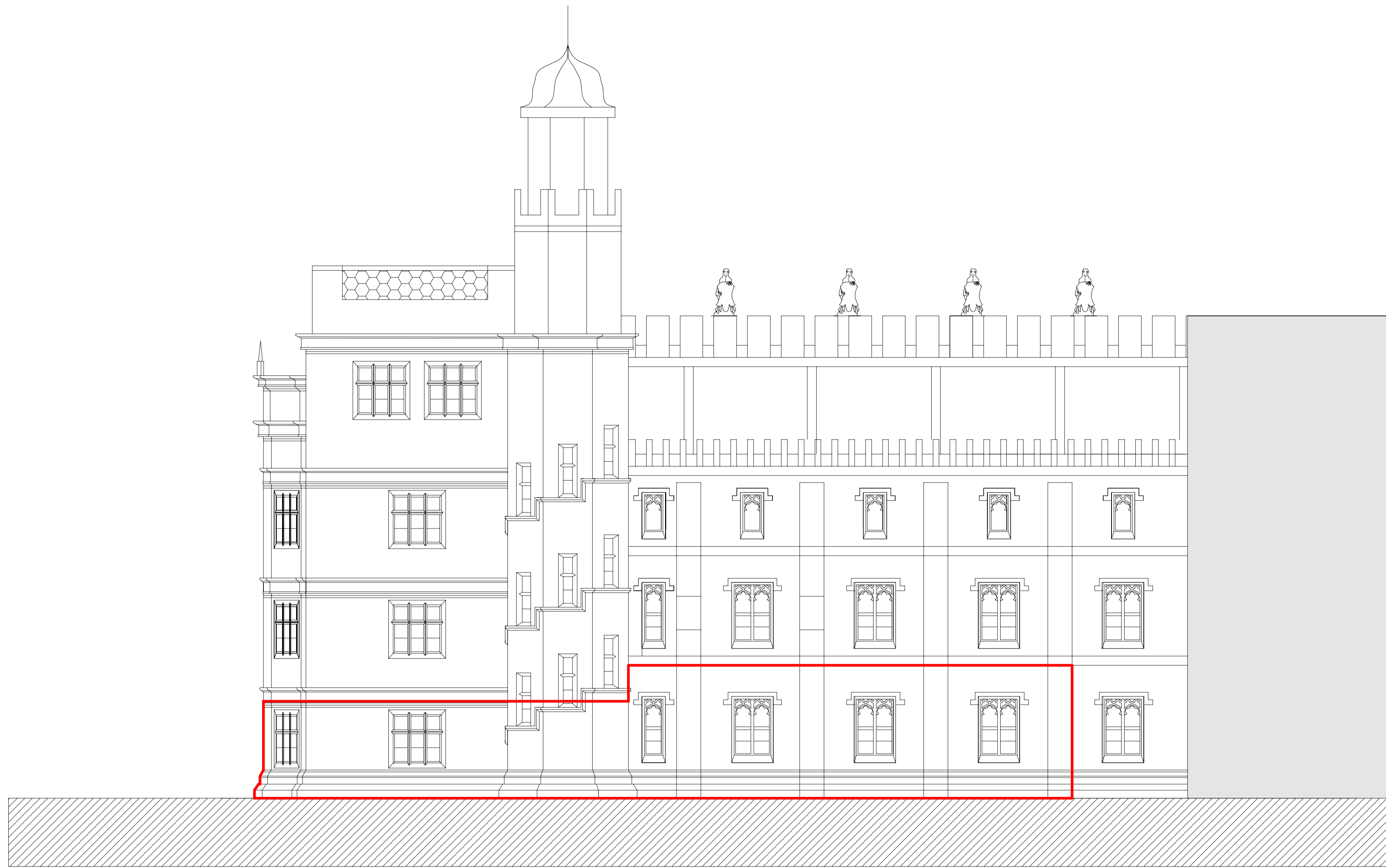
3 | Proposed East Elevation 1 : 100
