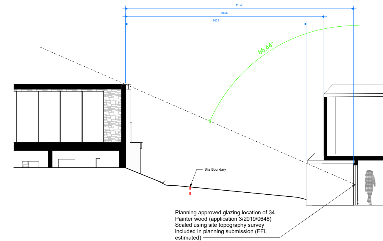
1 45 Degree Rule Section 1 : 50
