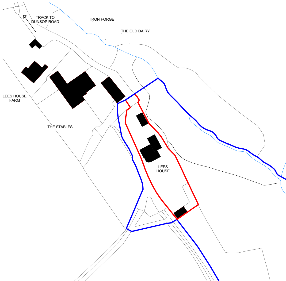
1 LOCATION PLAN 1 : 1250
