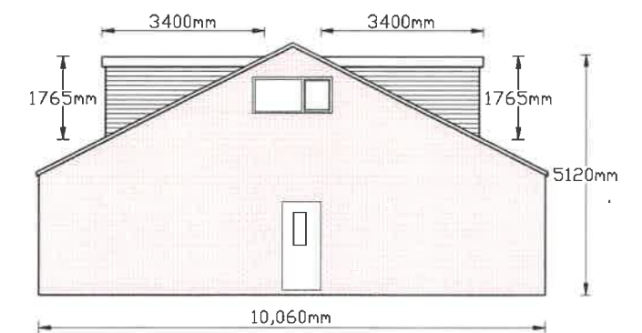
Side Elevation
