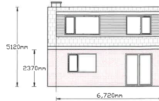
Rear Elevation
