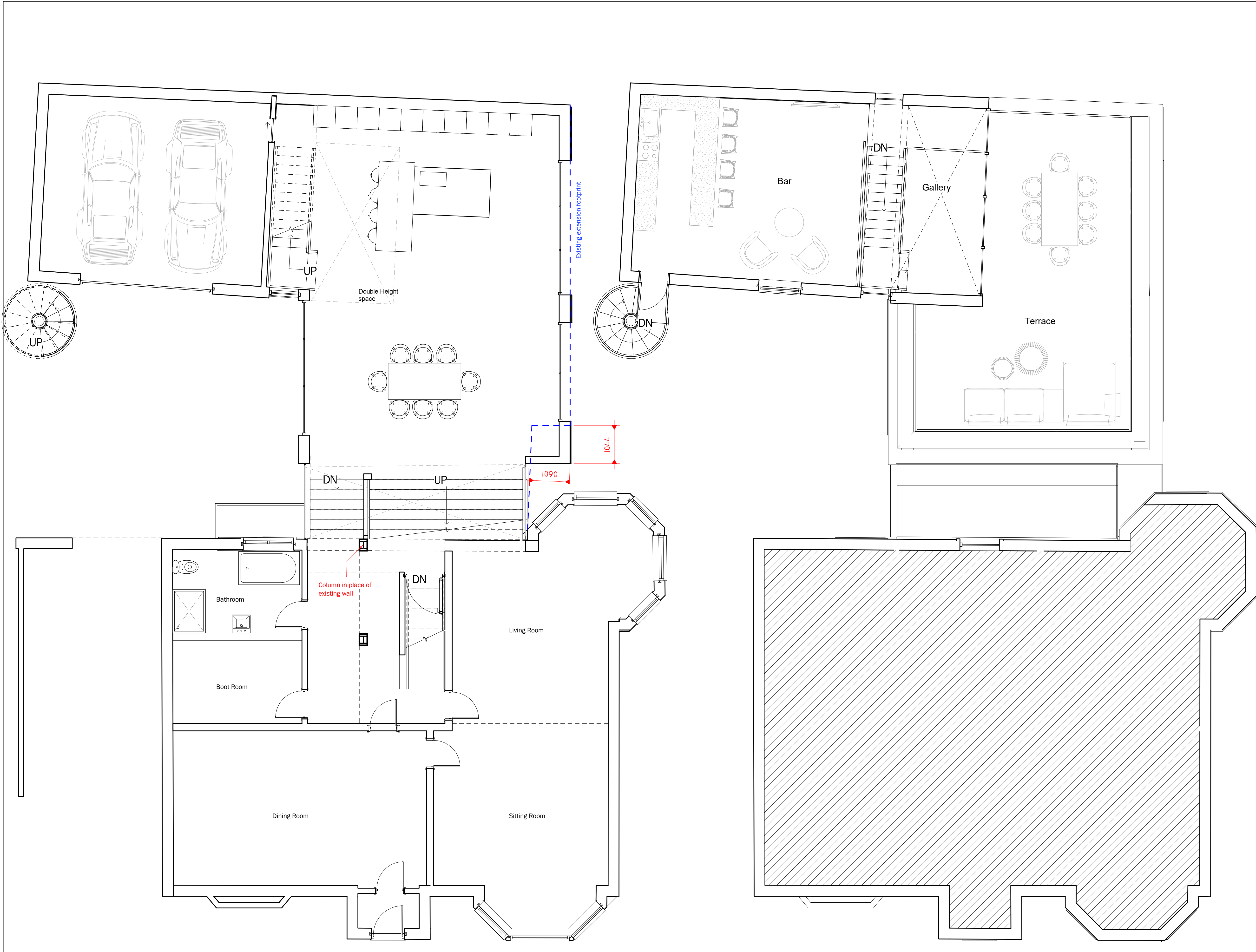
1 Kitchen Extension Floor 1 : 50
