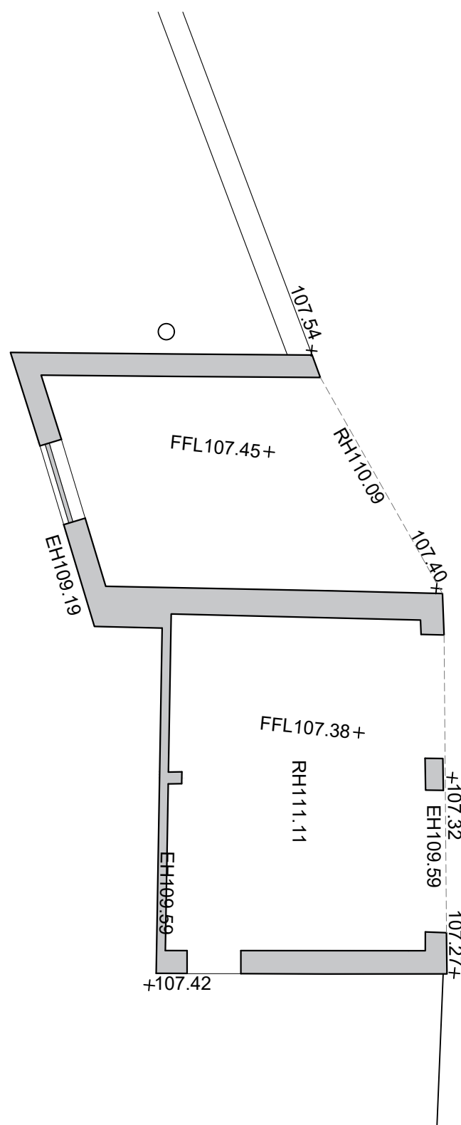
Outbuilding Floor Plan
