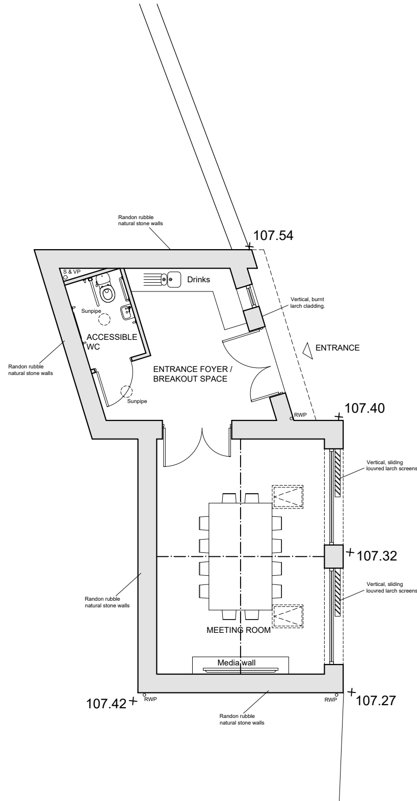
Outbuilding Floor Plan
