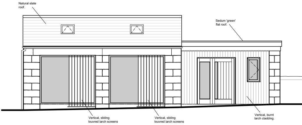
Outbuilding East Elevation
