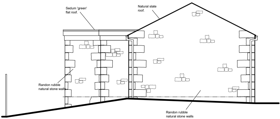
Outbuilding South Elevation
