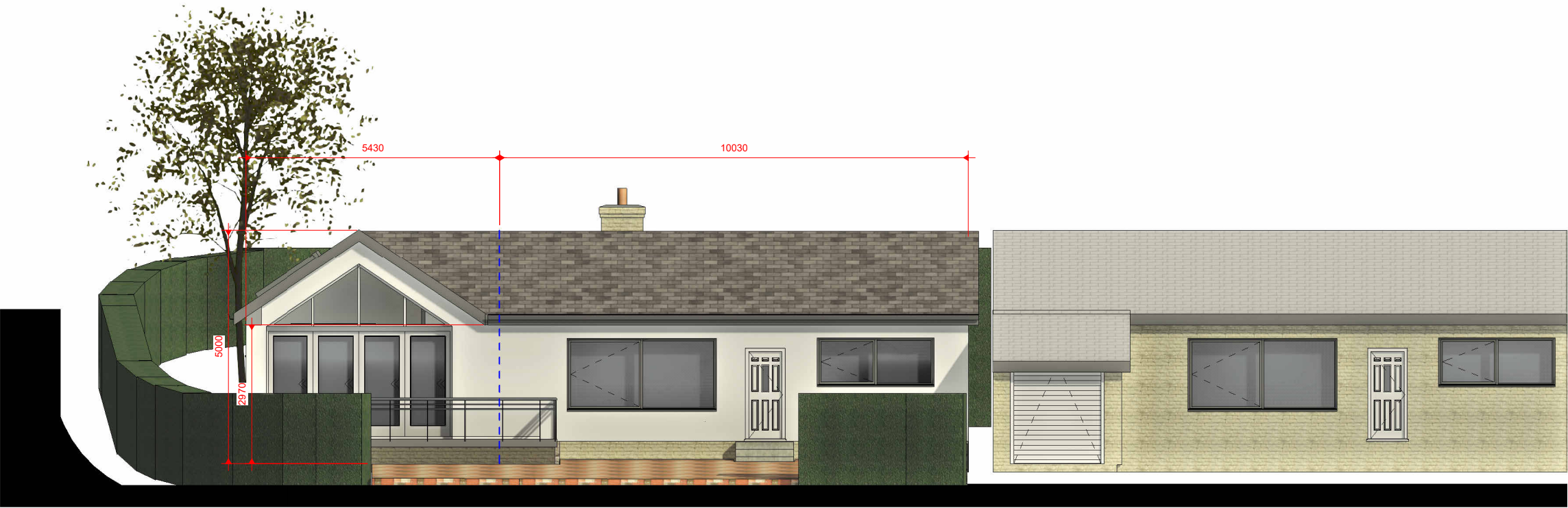
1 PROPOSED SOUTH 1 : 50
