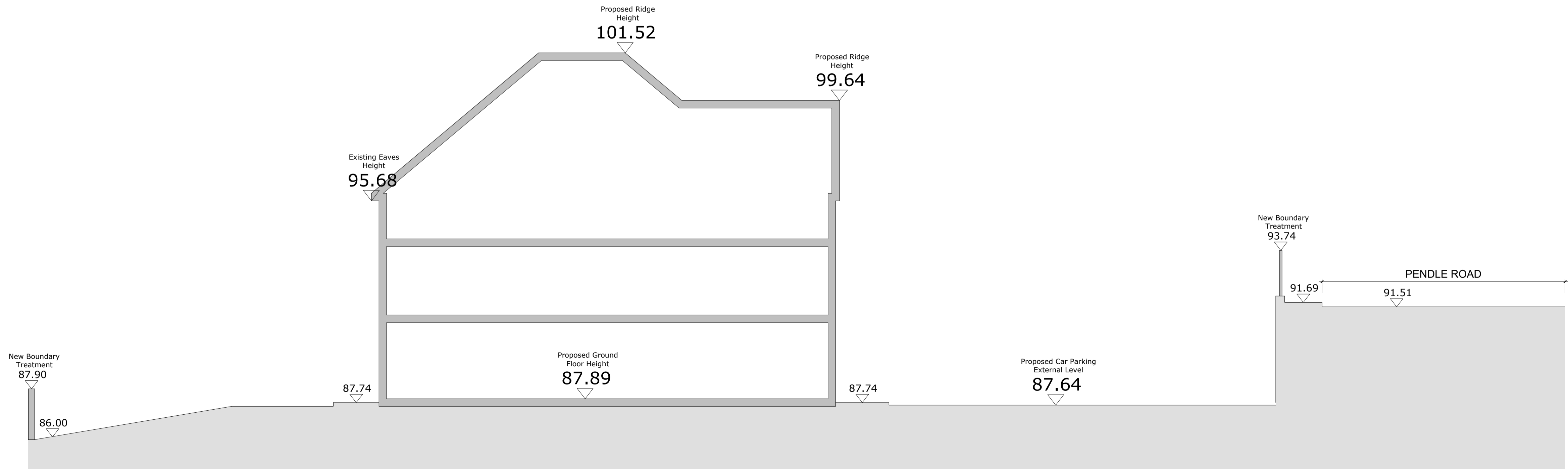
Proposed Site Section A-A
