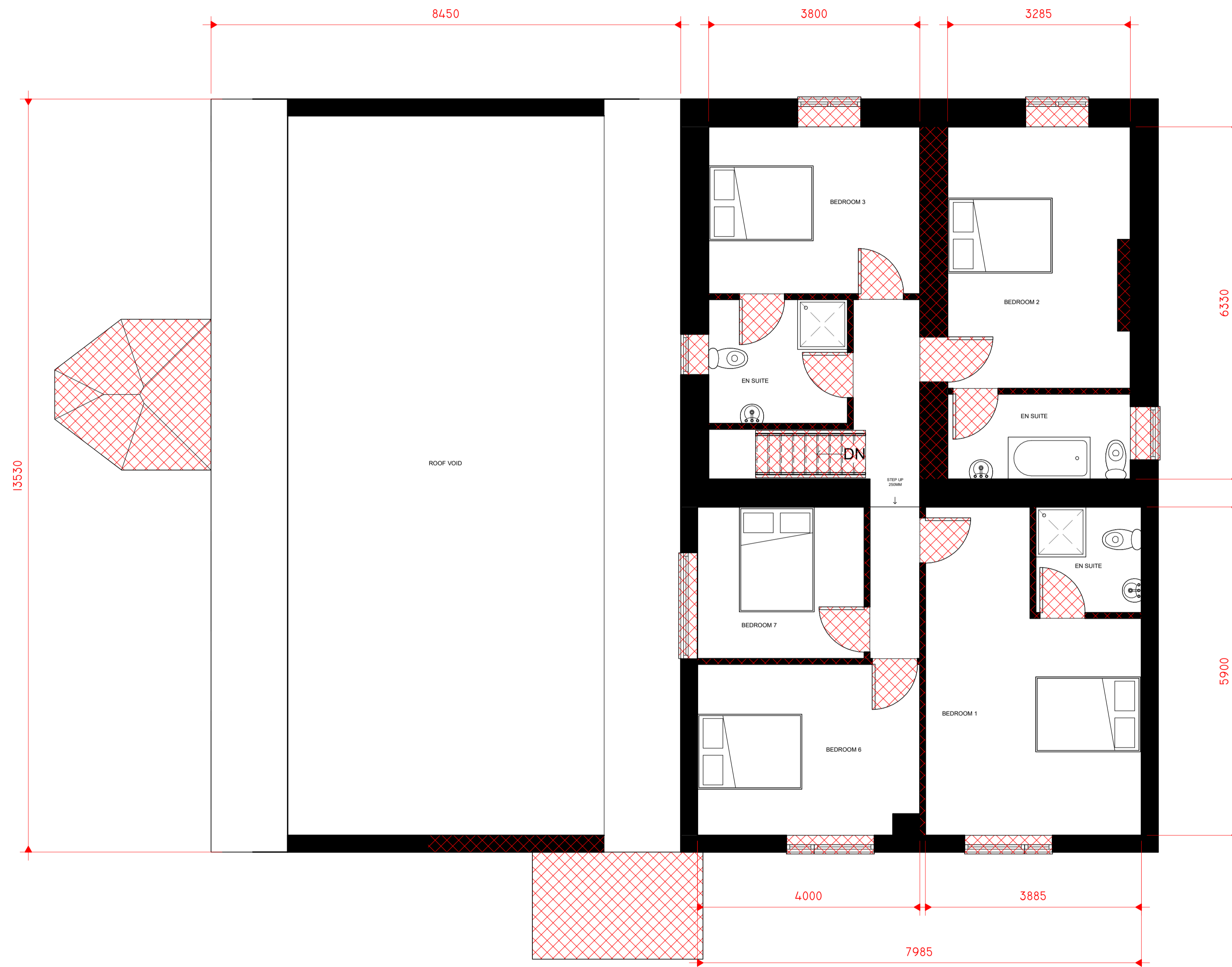
1 FIRST FLOOR DEMOLITION PLAN 1 : 50
