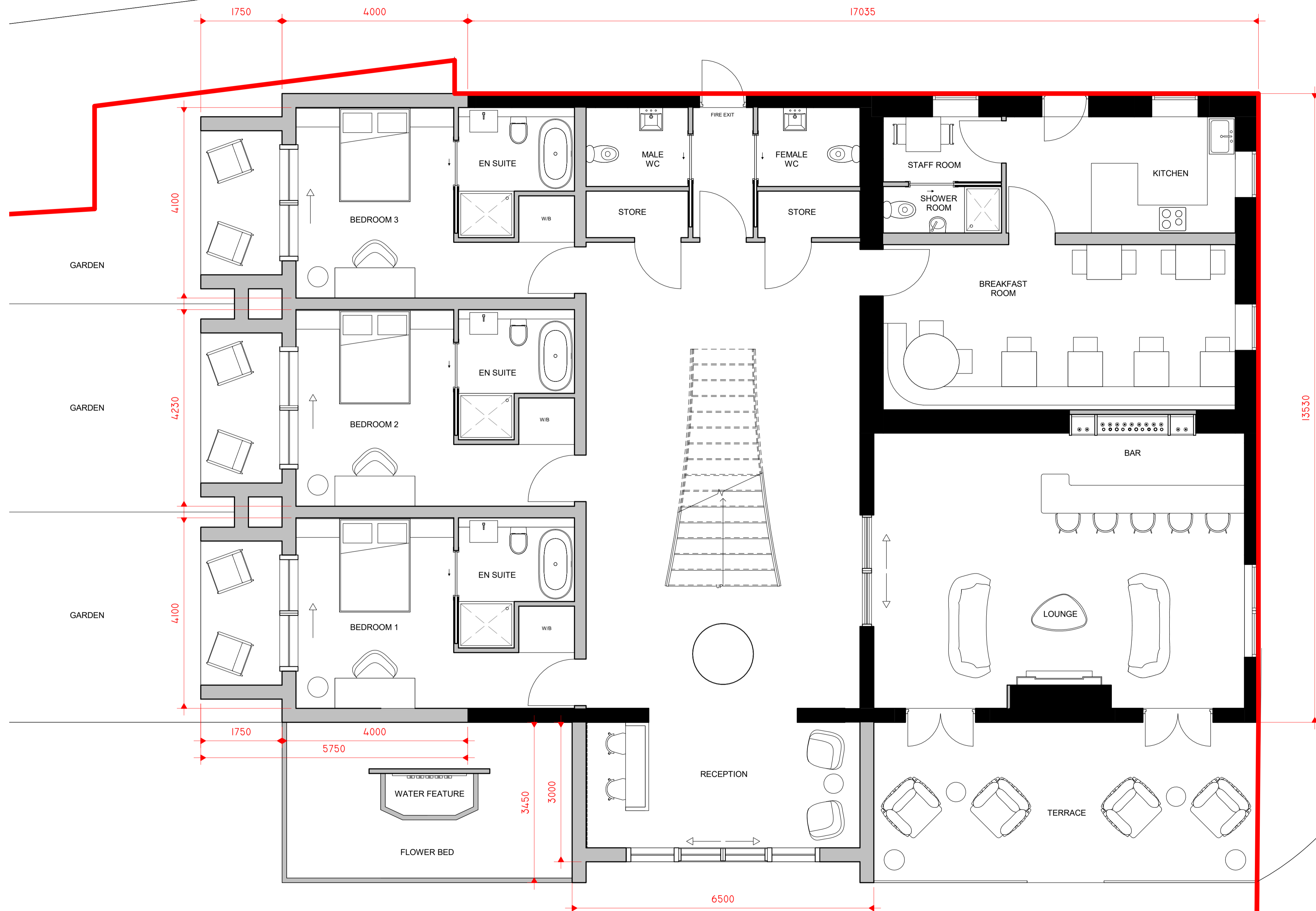
1 0 PROPOSED GROUND FLOOR 1 : 50
