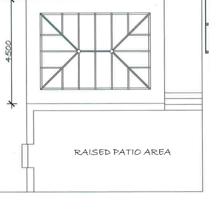
PROPOSED PLAN ELEVATION
