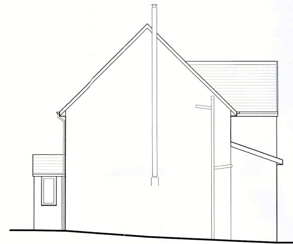
East Elevation
