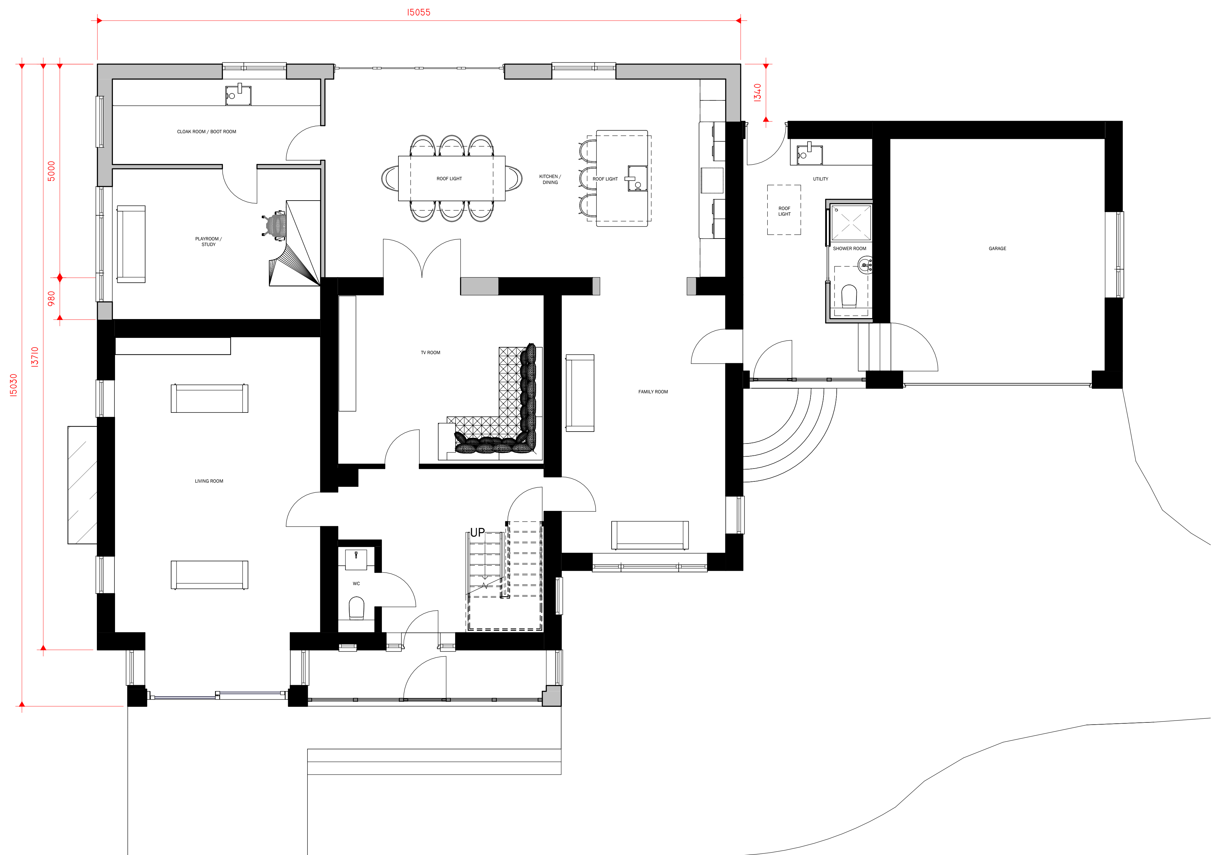
1 0 PROPOSED GROUND FLOOR 1 : 50
