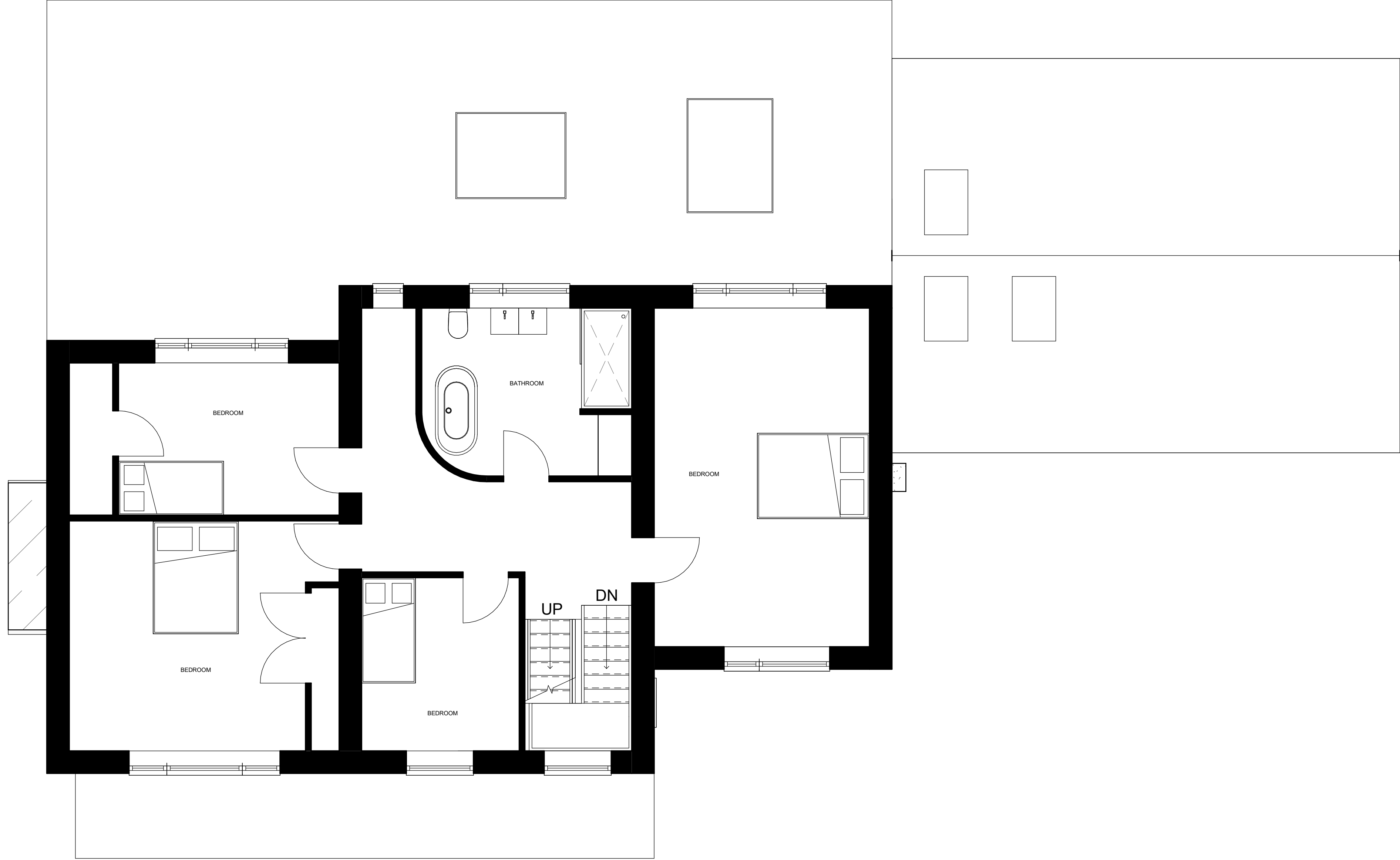
1 1 PROPOSED FIRST FLOOR 1 : 50
