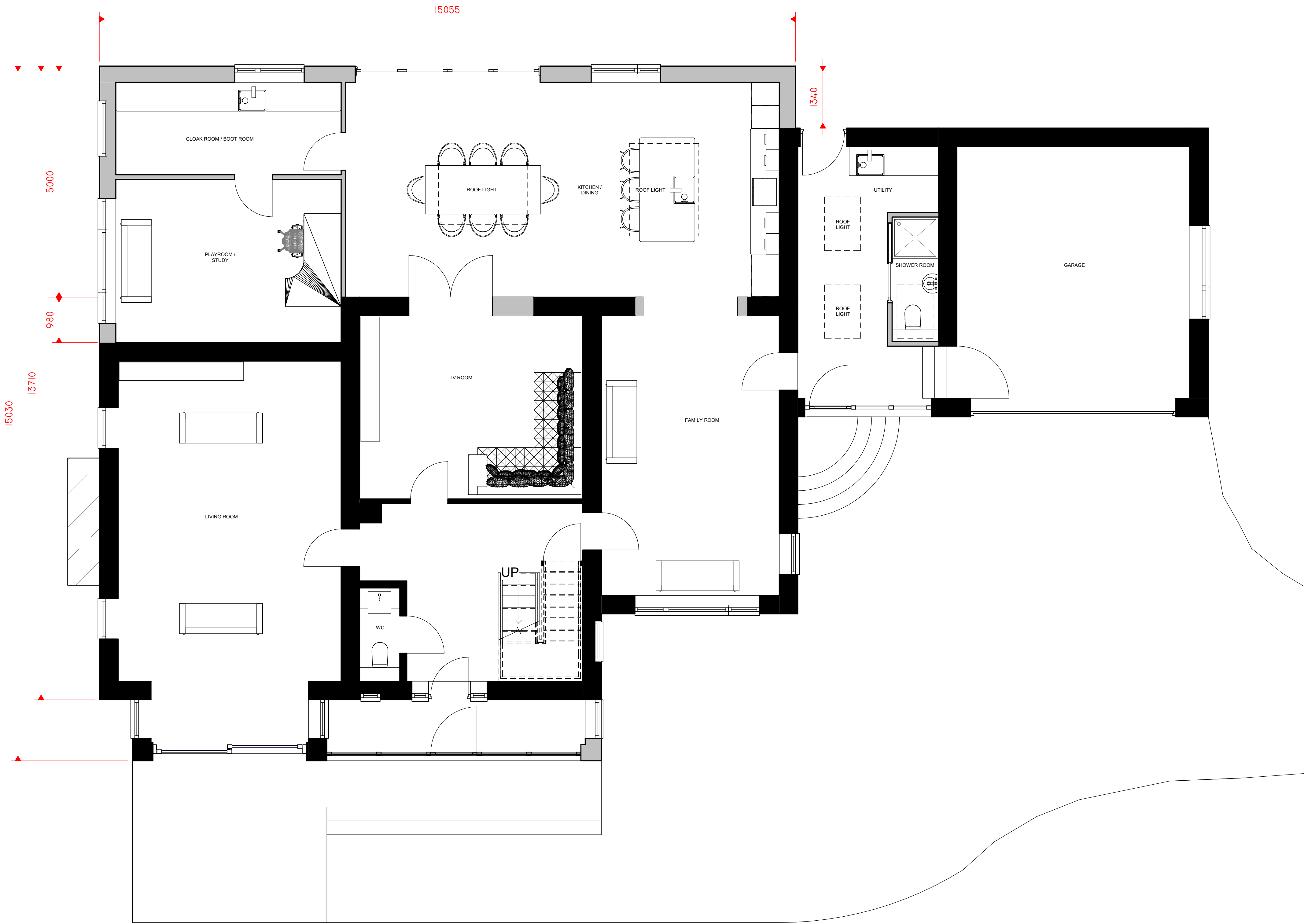
1 0 PROPOSED GROUND FLOOR 1 : 50
