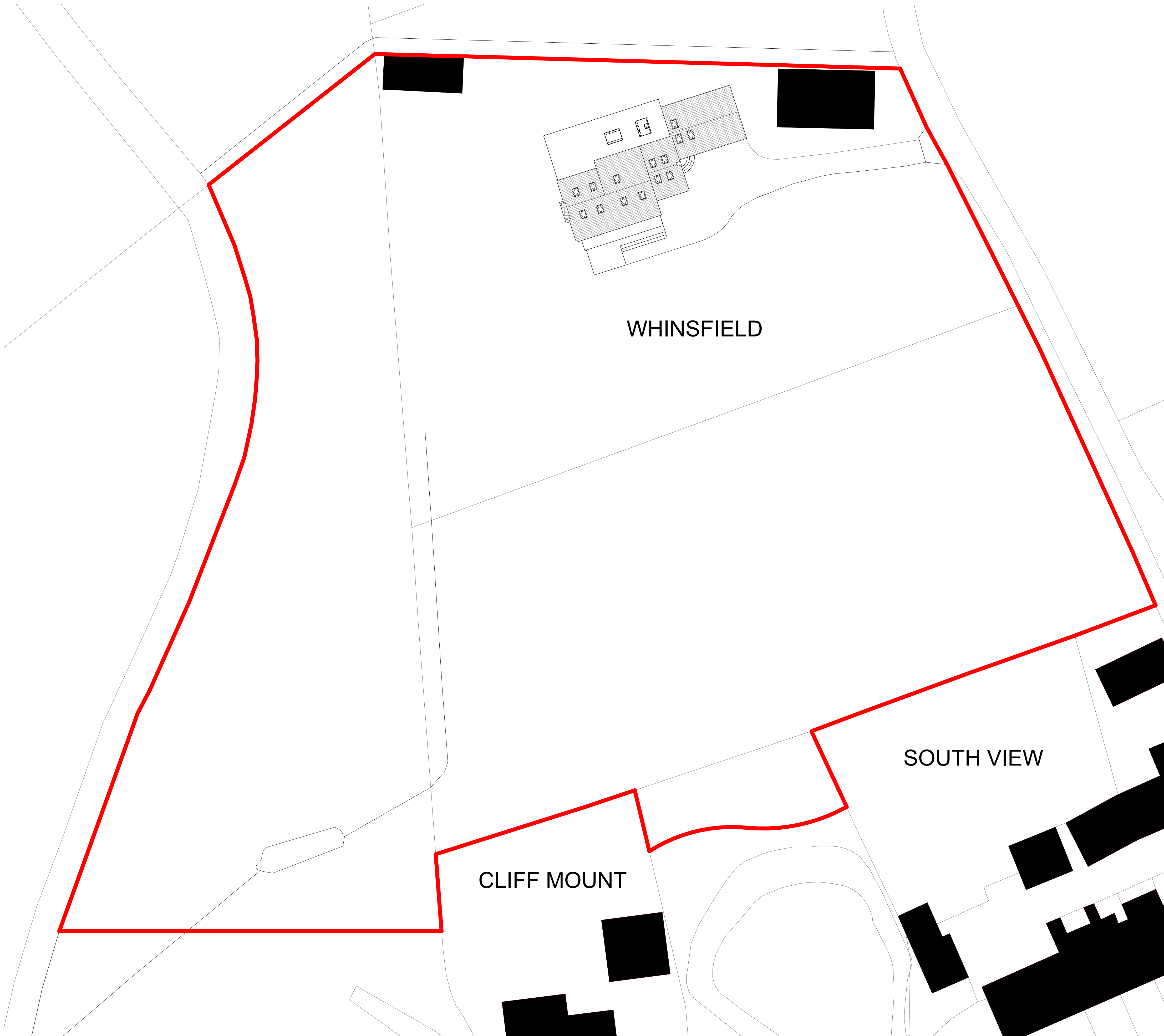
1 PROPOSED SITE PLAN 1 : 250
