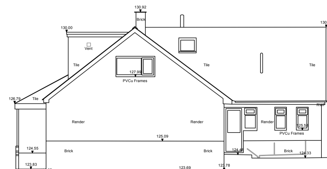
East Elevation
