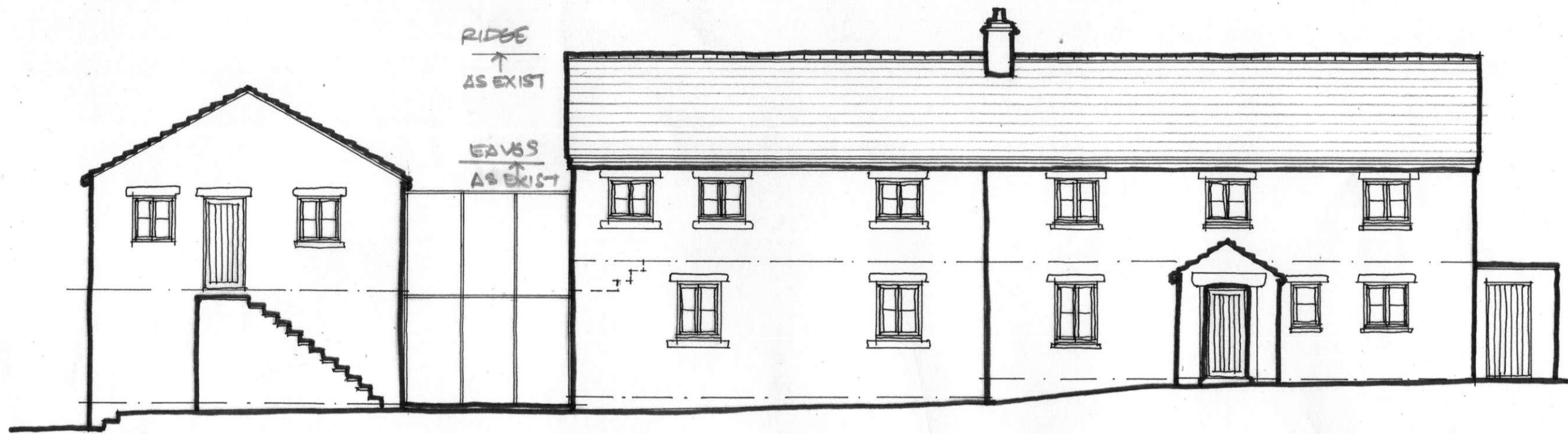
FRONT ELEVATION
