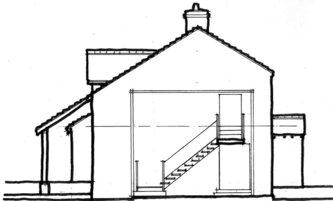
SECTION THRO' LINK B-B
