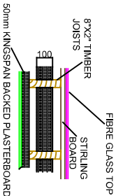
ROOF AND FRAME LAYOUT
