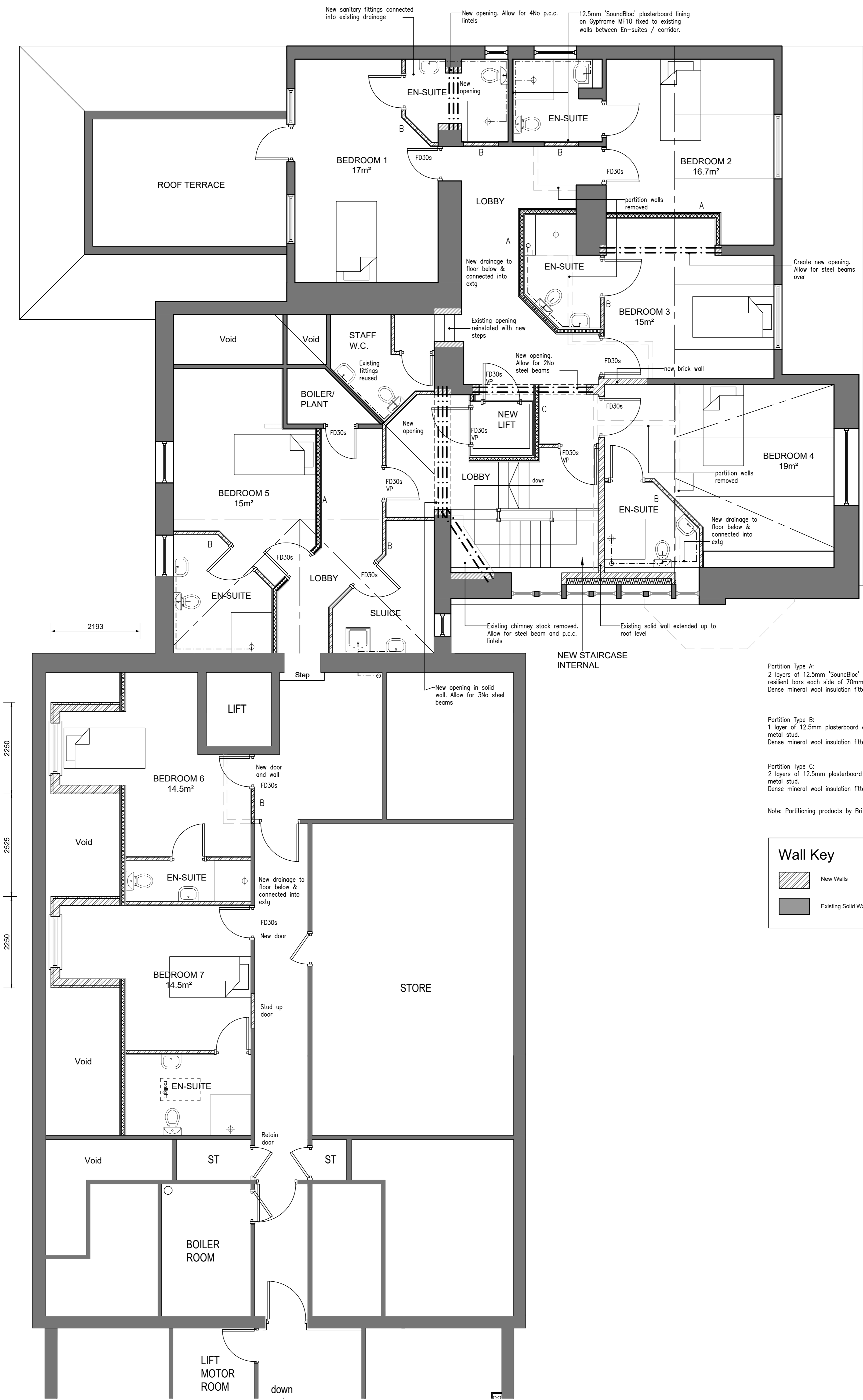
PROPOSED SECOND FLOOR LAYOUT 1:50
