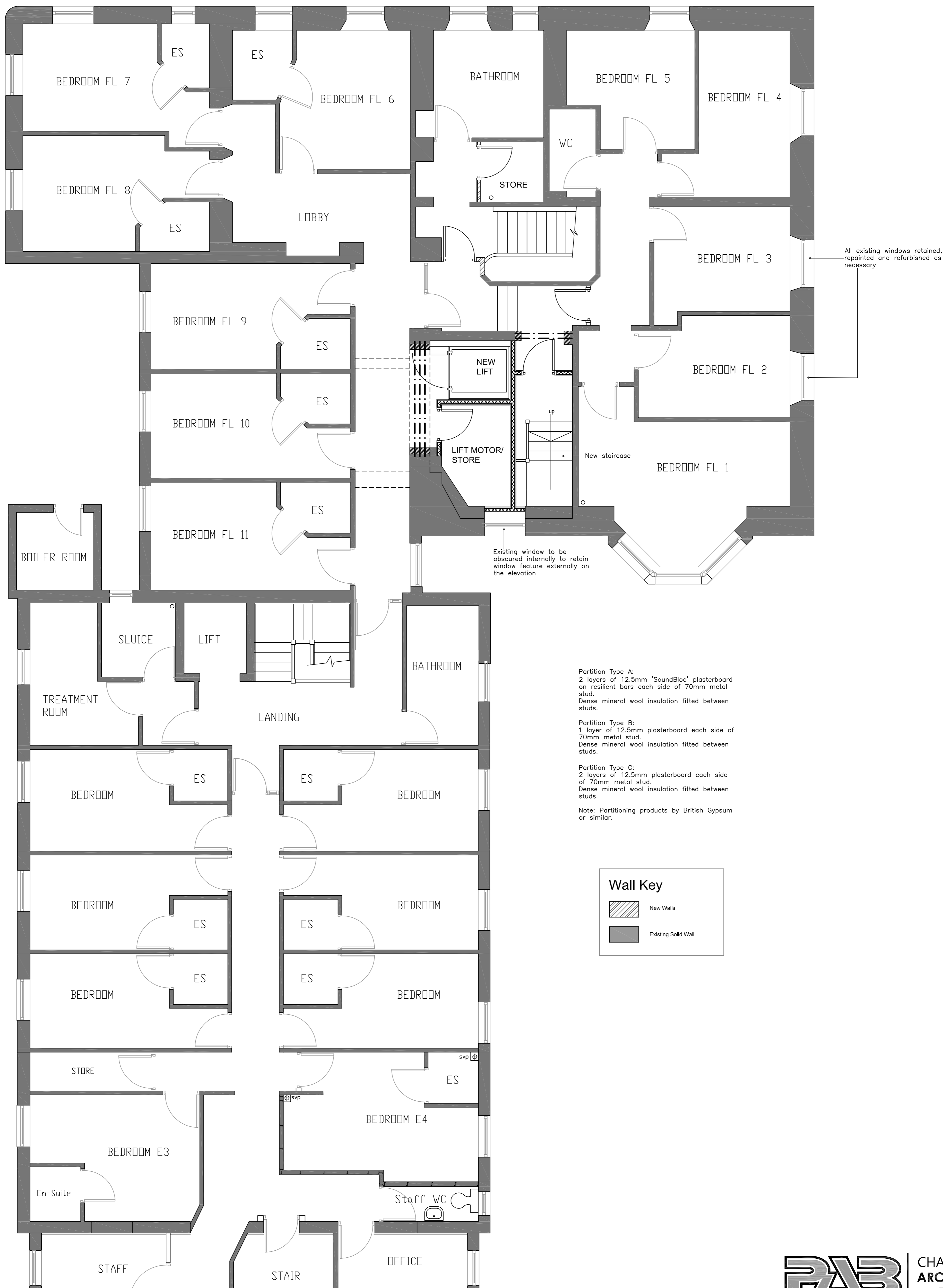
PROPOSED FIRST FLOOR LAYOUT 1:50
