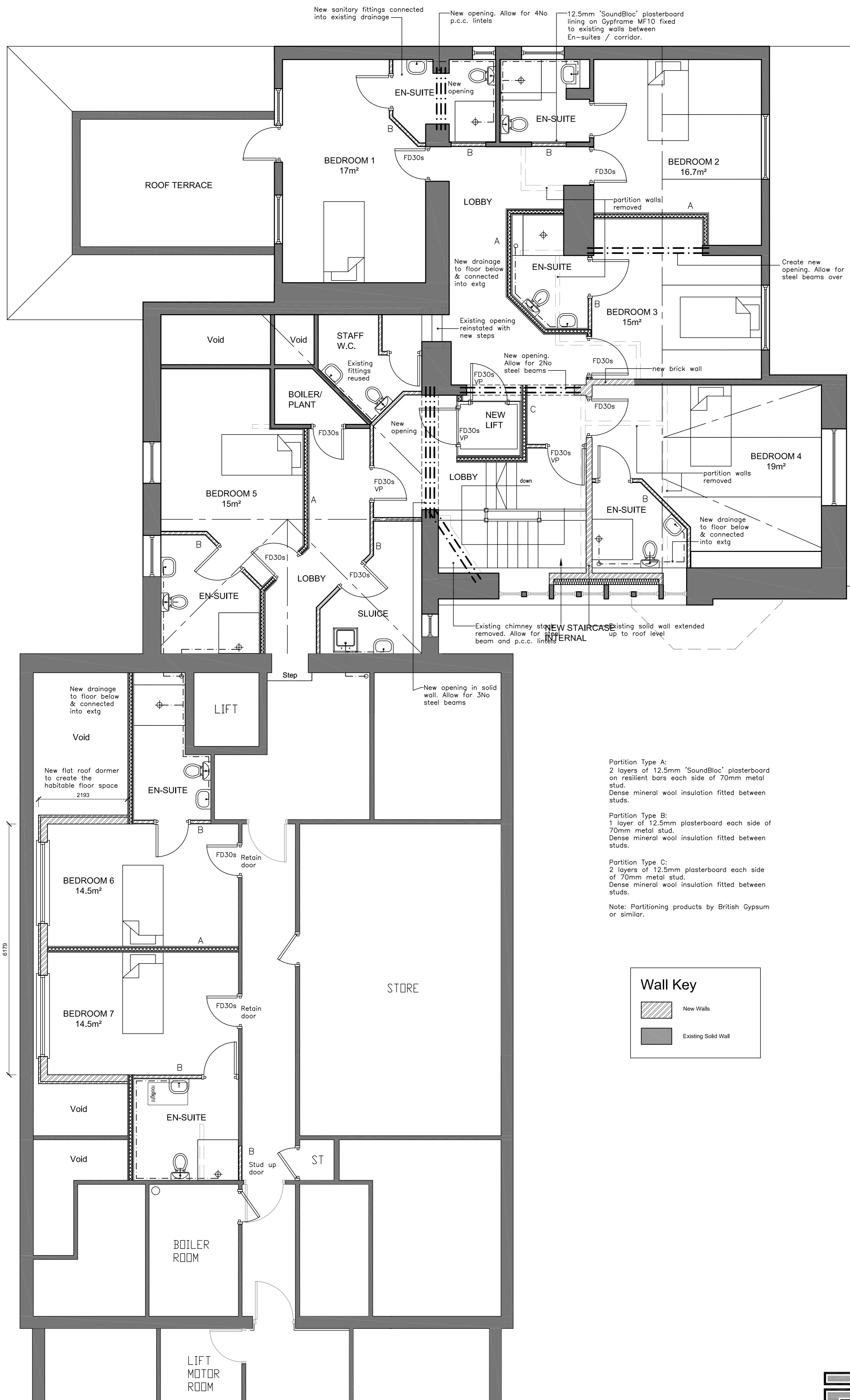
PROPOSED SECOND FLOOR 1:50
