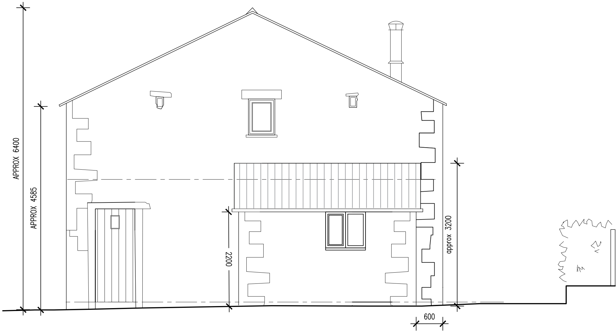
East Elevation
