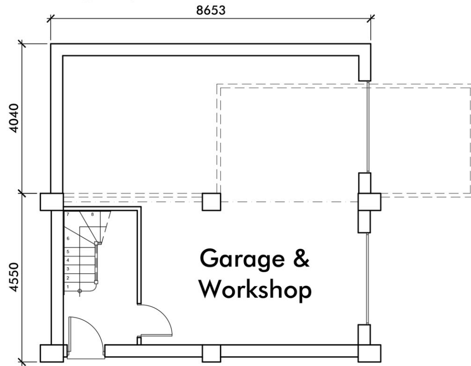
GF PLAN
