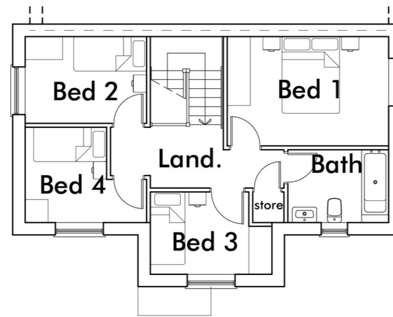
FF PLAN
