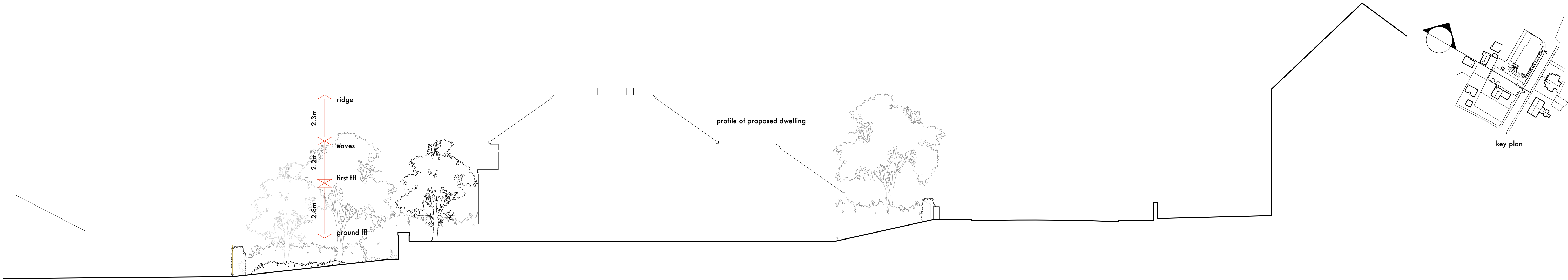
proposed site section
