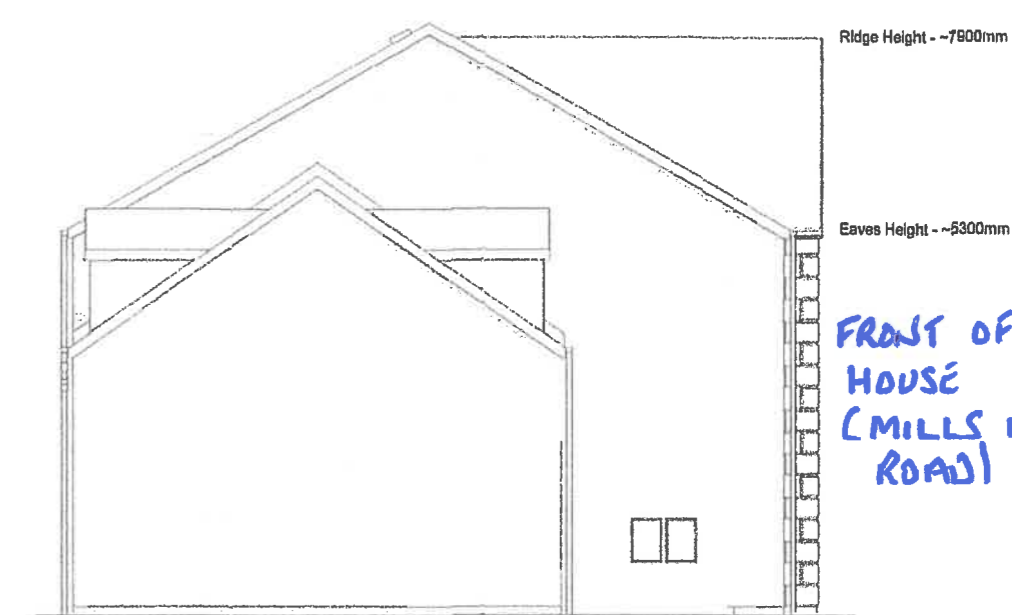
Left Elevation 1 : 100
