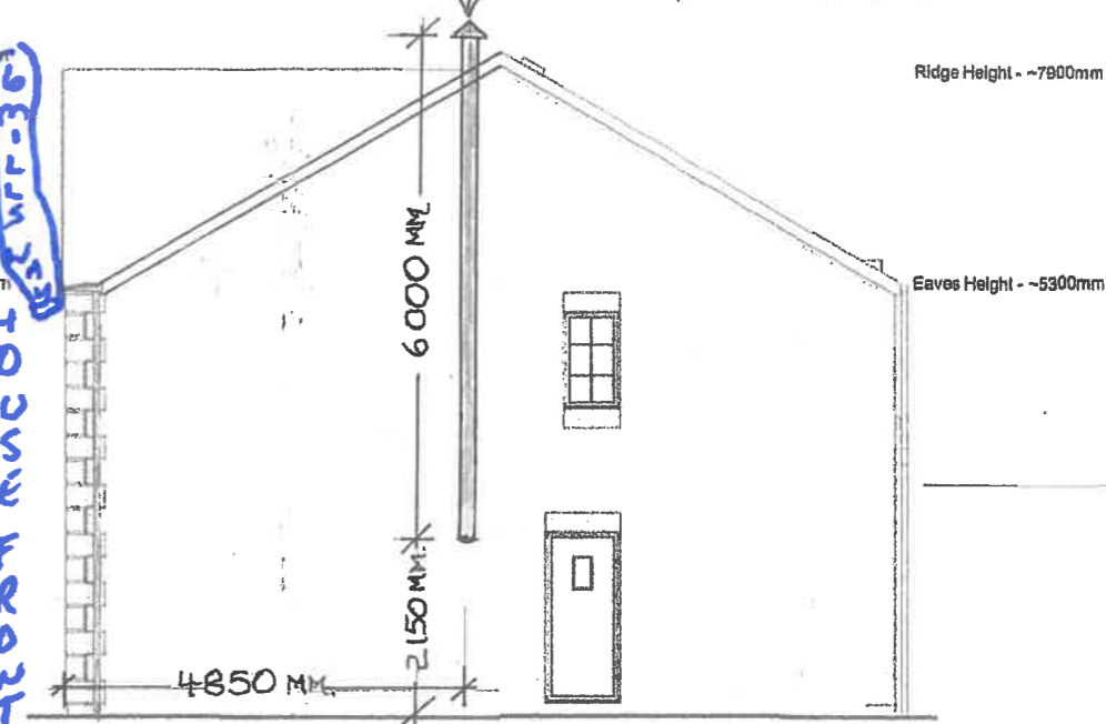
Right Elevation NORTH FACING 1 : 100
