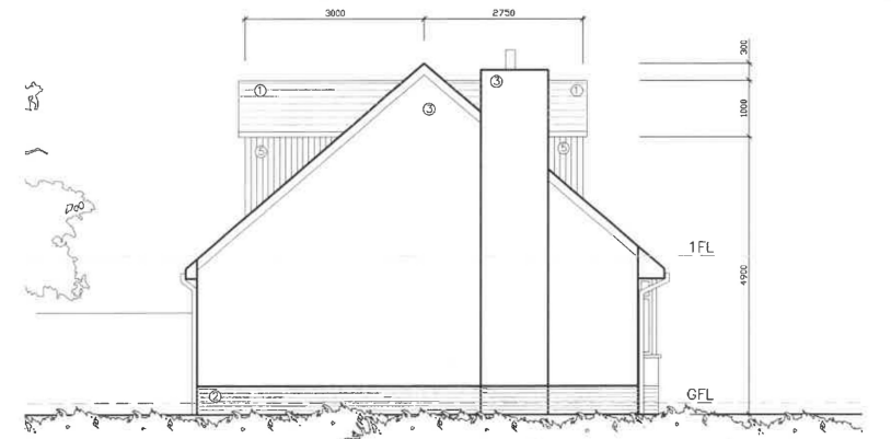
PROPOSED SOUTH ELEVATION (4)
