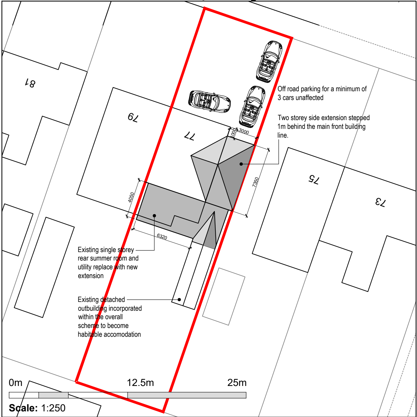
Proposed Site block plan - 1:250
