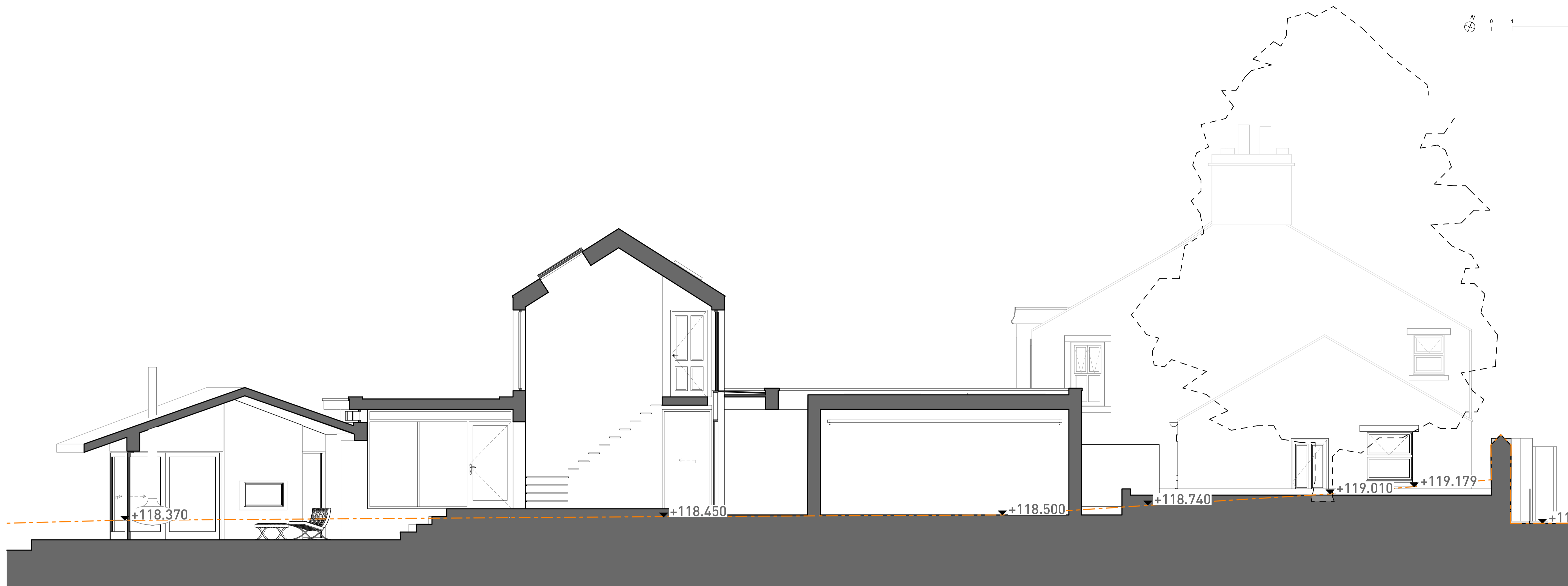
1 PROPOSED PART SECTION A-A Scale: 1:50
