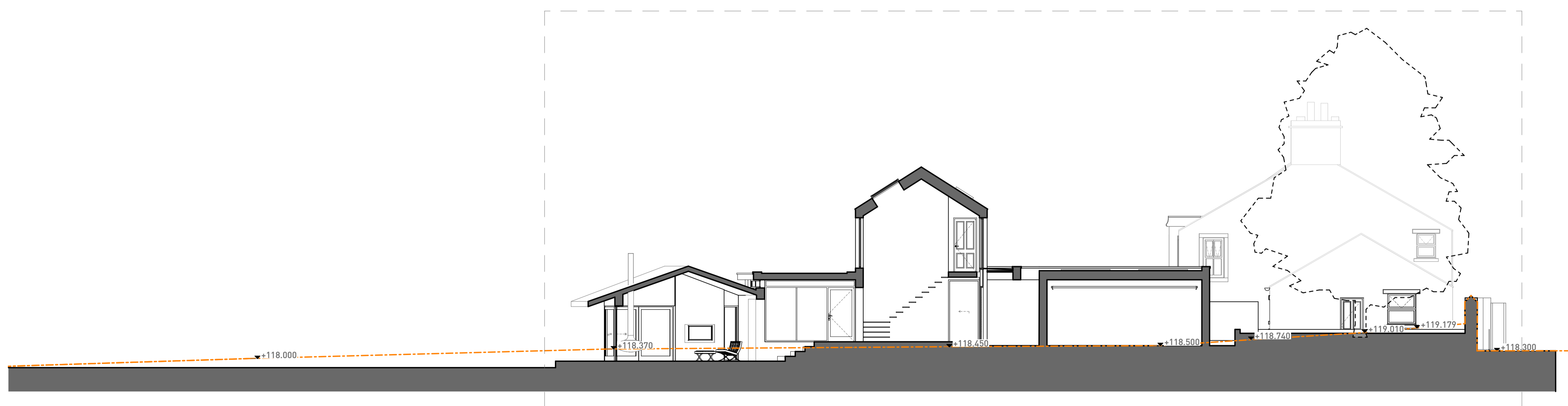
A-A PROPOSED SECTION A-A Scale: 1:100
